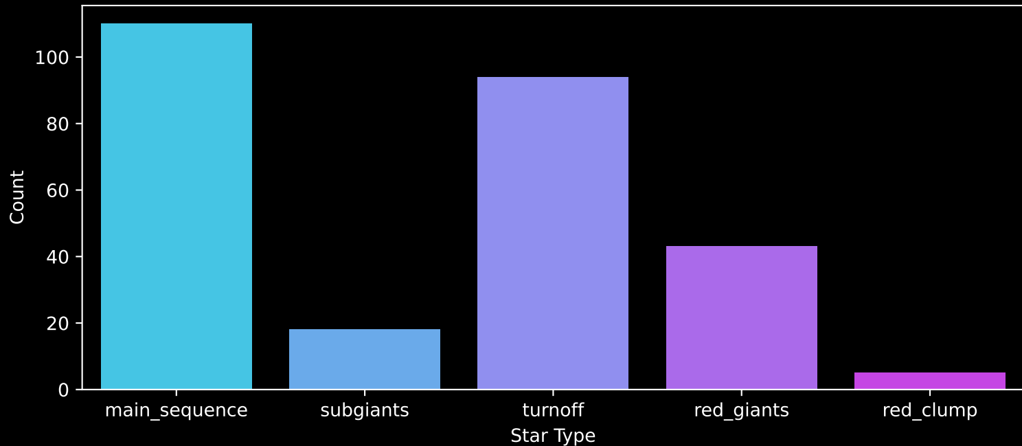
GALAH DR4 Field: [2485] Count plot of Star Type
