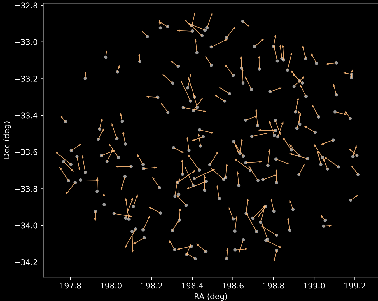
GALAH DR4 Cluster 3 Proper Motion Vectors (n=168)
