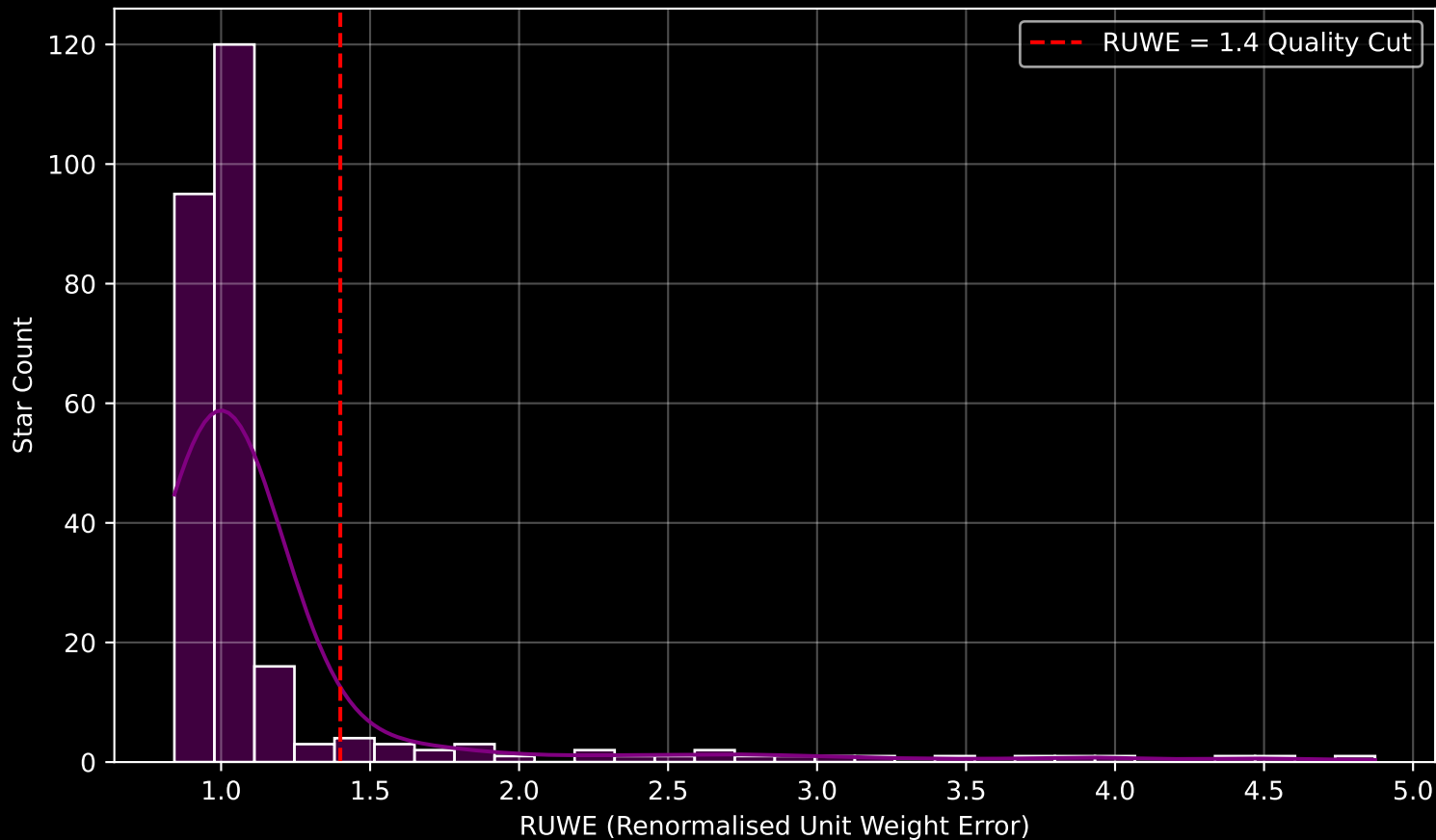
GALAH DR4 Field [2485] RUWE Distribution (n= 264)
